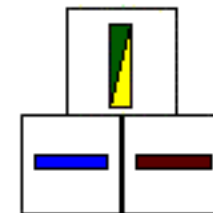
EARTH = GREEN/YELLOW AC NEUTRAL = BLUE AC LIVE = BROWN HARNESS SOCKET (FEMALE)
